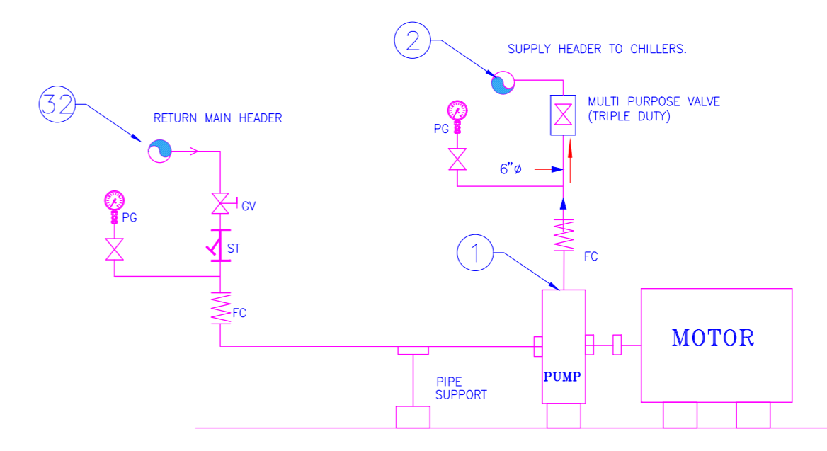
CHILLED WATER PUMP PIPING CONNECTIONS NOT TO SCALE
