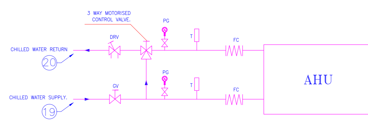
AHU PIPING CONNECTIONS NOT TO SCALE
