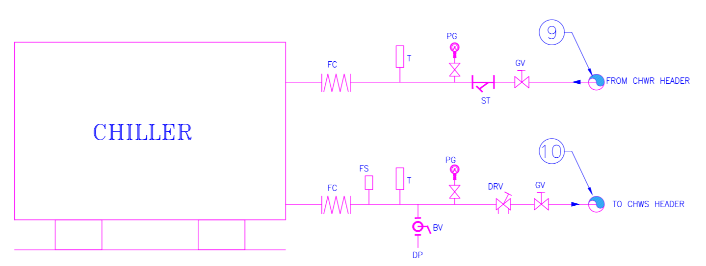
CHILLER PIPING CONNECTION NOT TO SCALE
